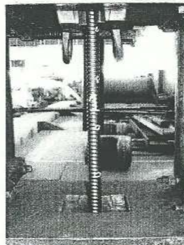
Photo 1: R32S Self drilling anchor installed in the testing machine.
